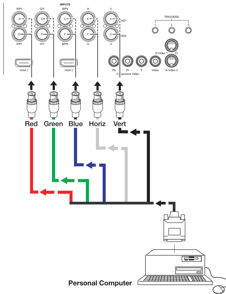
Figure 3-11. Analog RGB Connections
